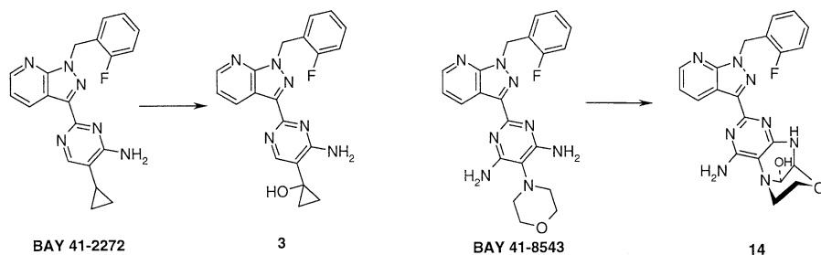
Scheme 1. Main metabolites of BAY 41-2272 and BAY 41-8543 in rats and dogs.
